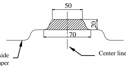
Fig. 3 Bumper cut out Mazda Tribute
