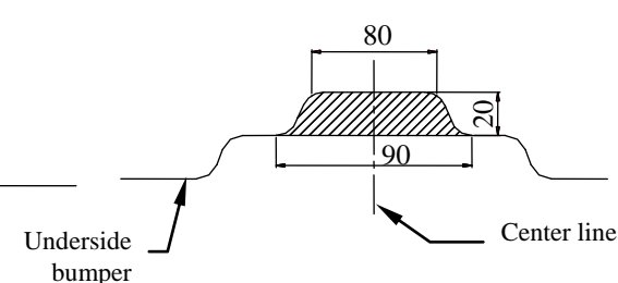
Fig. 3 Bumper cut out Mazda Tribute
